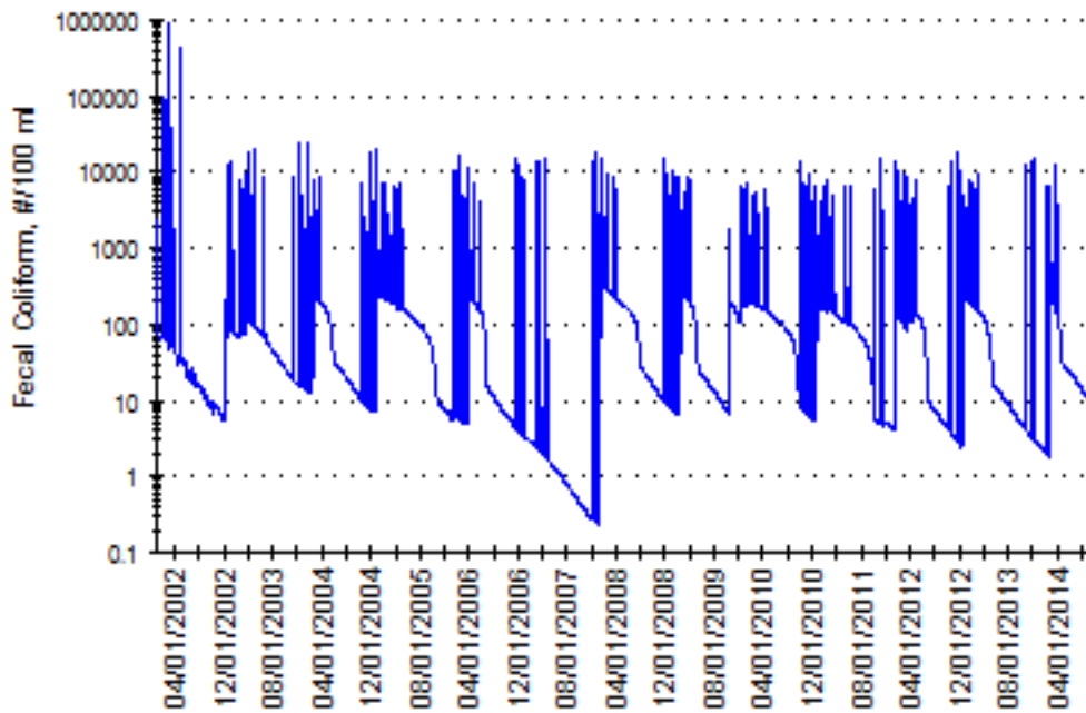
Figure 52. Modeled E. coli concentrations (MPN/mL) in catchment 1 from 2002 to 2014. No observed data available in this catchment.
