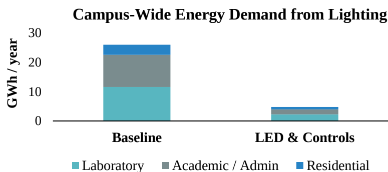
Figure 10. Campus-wide Energy Demand from Lighting (Baseline vs. LED & Controls).
