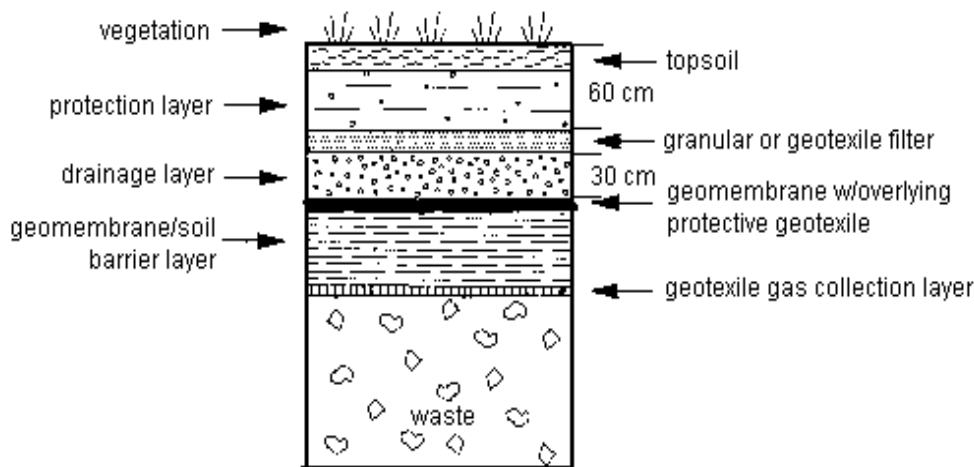
Figure 10: Typical design of a containment cap (FRTR, 2002)
