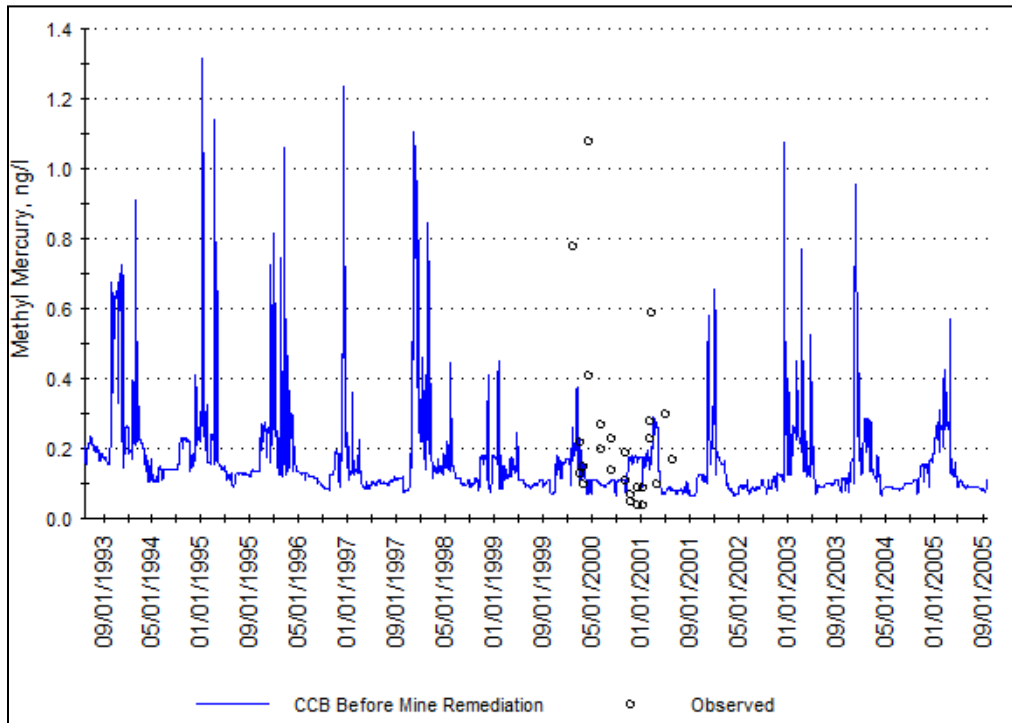
Figure 58: Modeled vs. observed methylmercury at Rumsey
