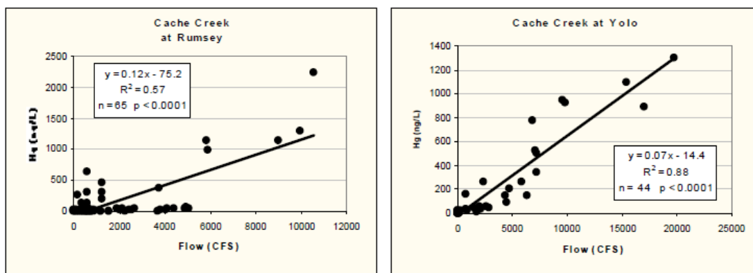
Figure 41: Linear regressions of mercury vs. flow at Rumsey and Yolo (Cooke, et al., 2004)
