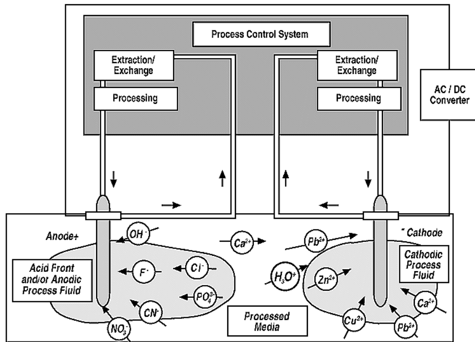
Figure 11: Electrokinetic System (FRTR, 2002)
