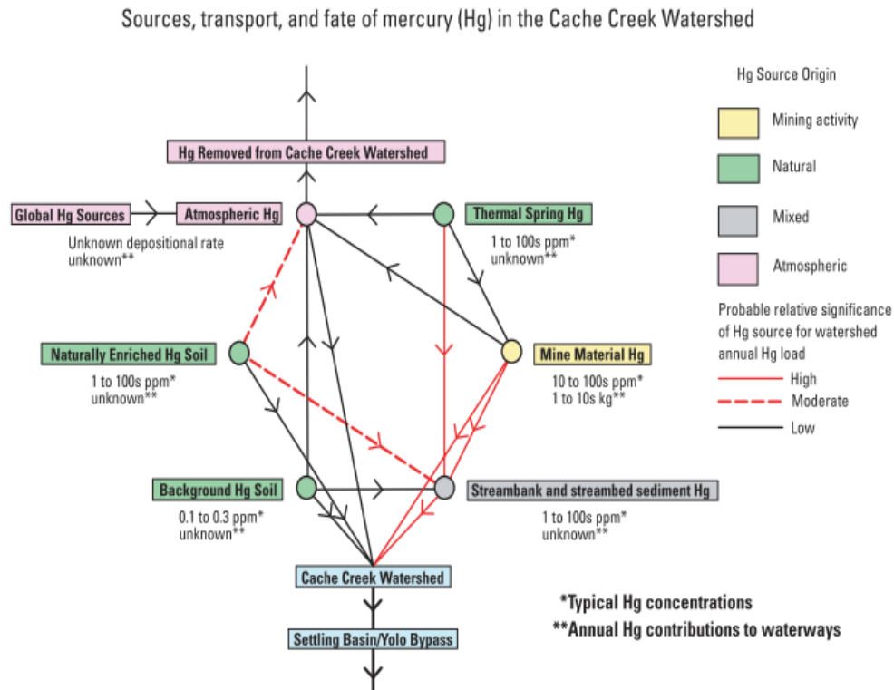
Figure 8: Sources, transport and fate of mercury in the Cache Creek watershed (Domagalski et al., 2004b)
