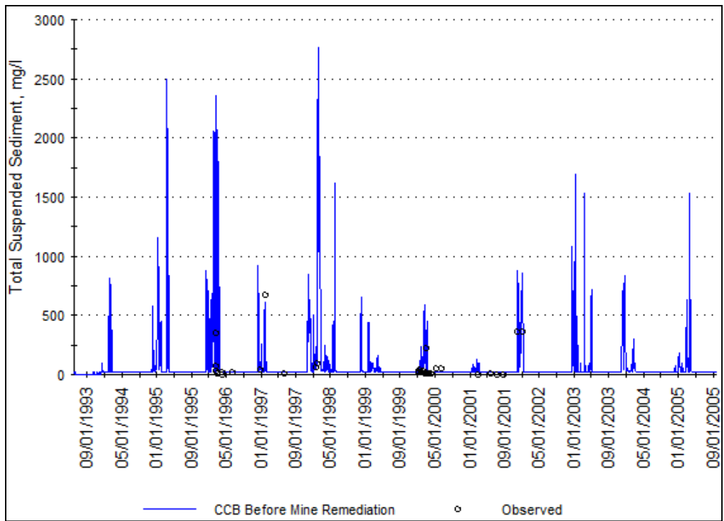
Figure 59: Modeled vs. observed suspended sediment, Bear Creek
