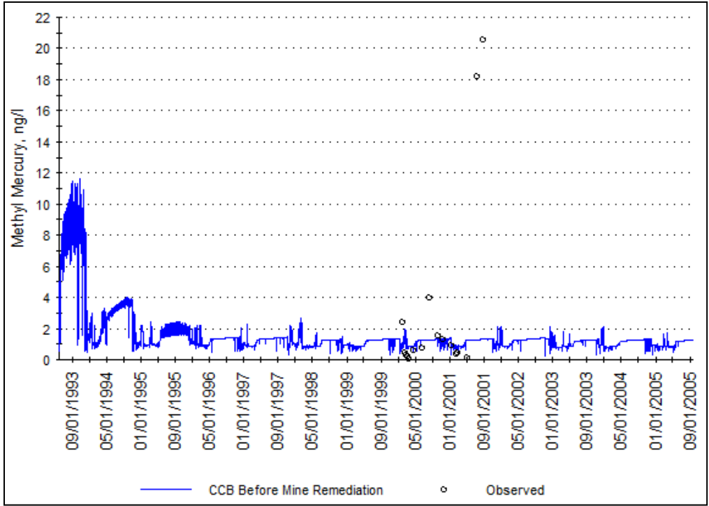
Figure 63: Modeled vs. observed methylmercury in Sulphur Creek.
