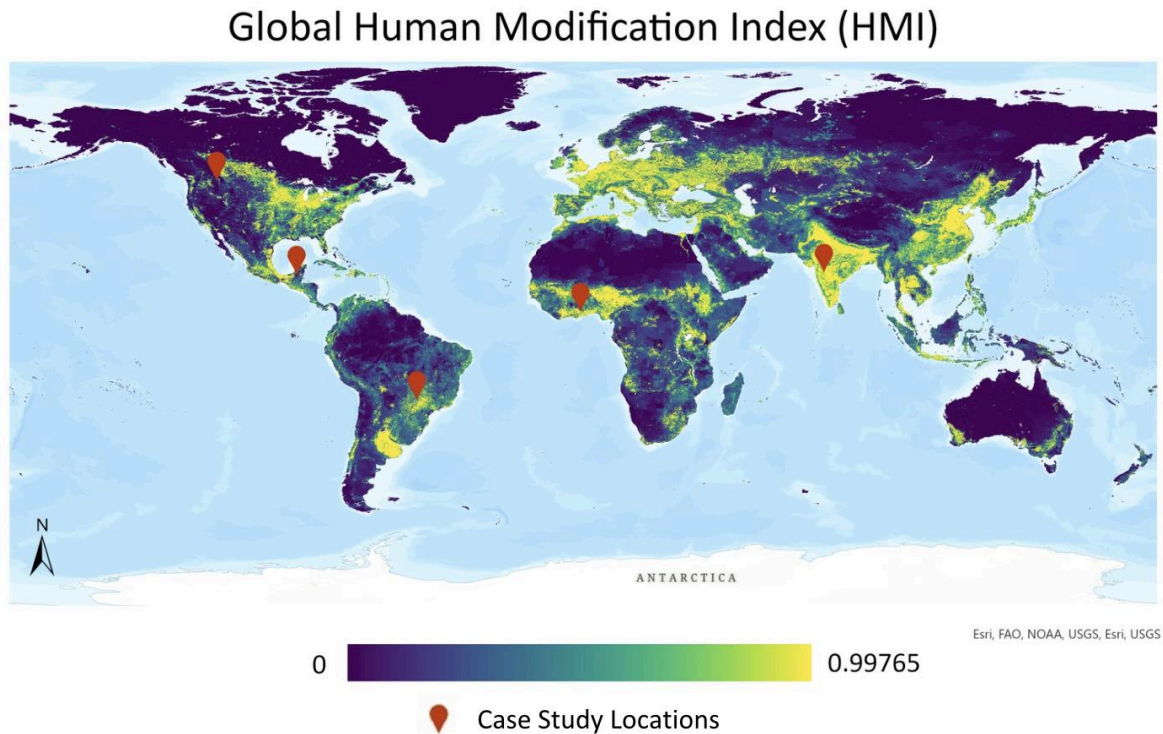
Figure 9. Map showing the global distribution of HMI values. Darker colors have values closer to 0 while lighter colors have values closer to the global maximum of 0.99765.
